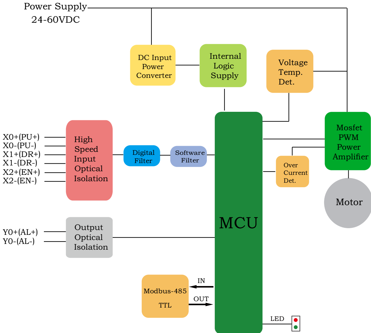
IG57ET Block Diagram
