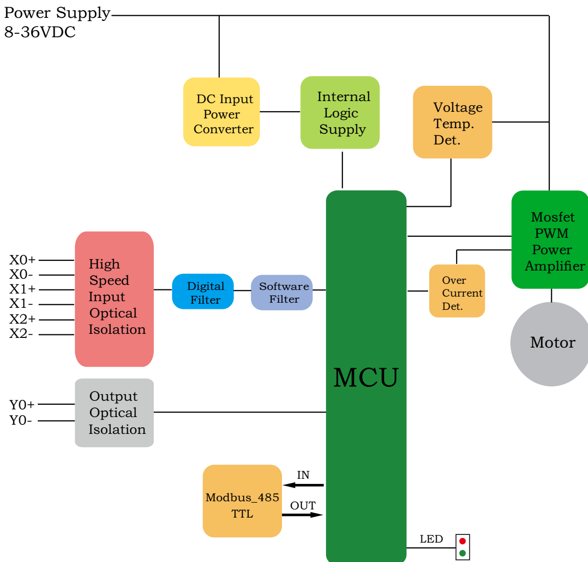
IG28ET Block Diagram
